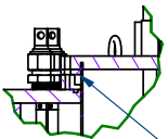
DETAIL B SCALE 1/5 TEFLON SLIDING SEAL
